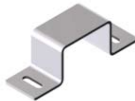
20075 Connection bracket. Fully zinc plated. Designed to mount the beam onto the triangle bracket. Also for mounting bearing plate or spring break device.
